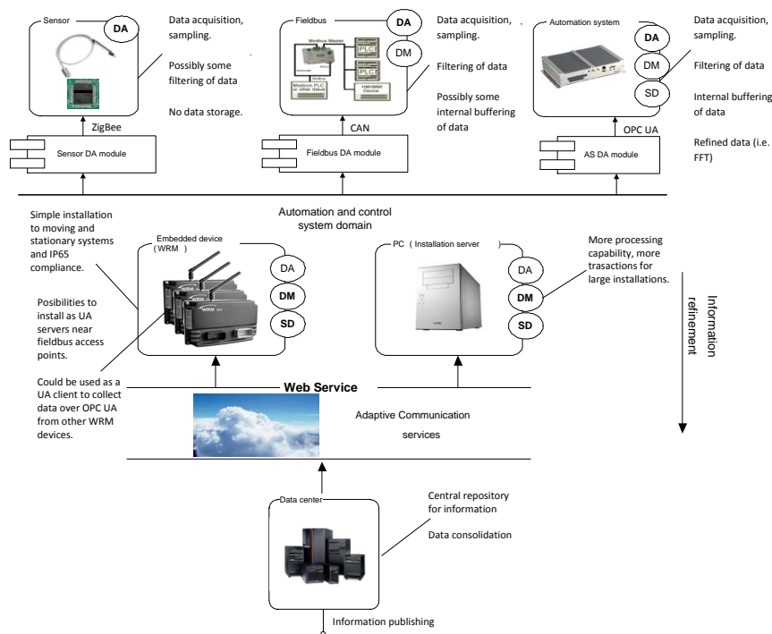
Figure 2. WRM Remote Management Platform.
