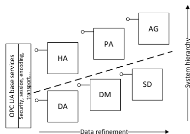
Figure 1. MIMOSA and OPC UA integration and system hierarchies.
